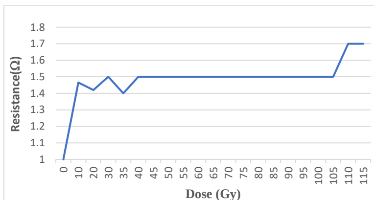
Figure 7. low Resistances in Ohm vs 6 MeV electron doses
