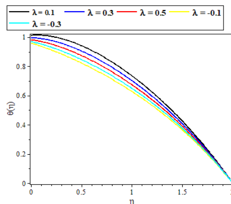
Figure 4: Influence of heat generation/absorption on temperature profile.
