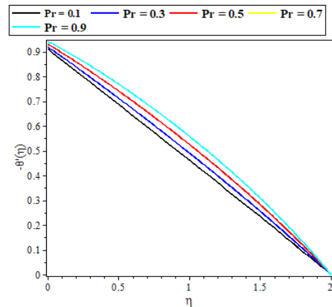
Figure 6: Influence of Prandtl number on Nusselt number profile.
