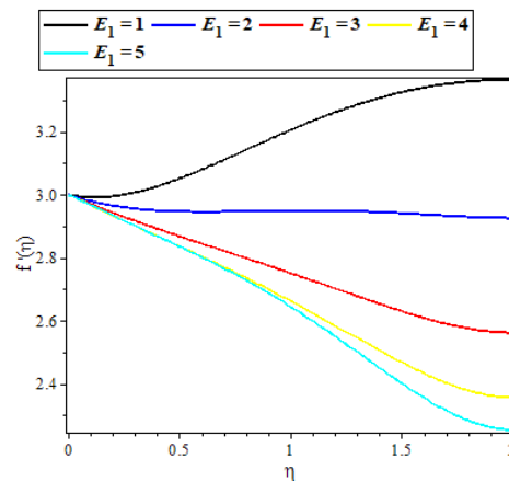
Figure 3: Influence of Electricity parameter on momentum profile.
