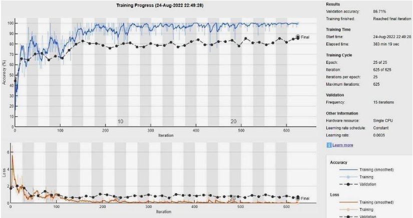
Figure 10: Training Graph of ResNet-101
