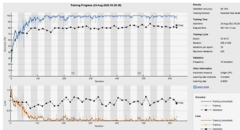
Figure 14: Training Graph of Inception-ResNet-V2
