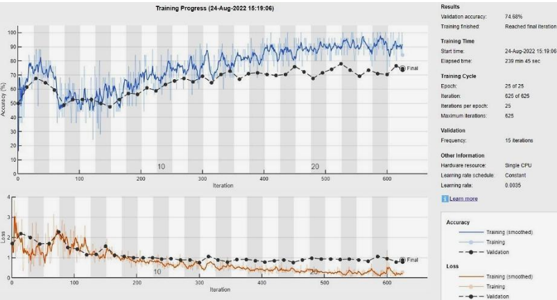
Figure 9: Training Graph of ResNet-50
