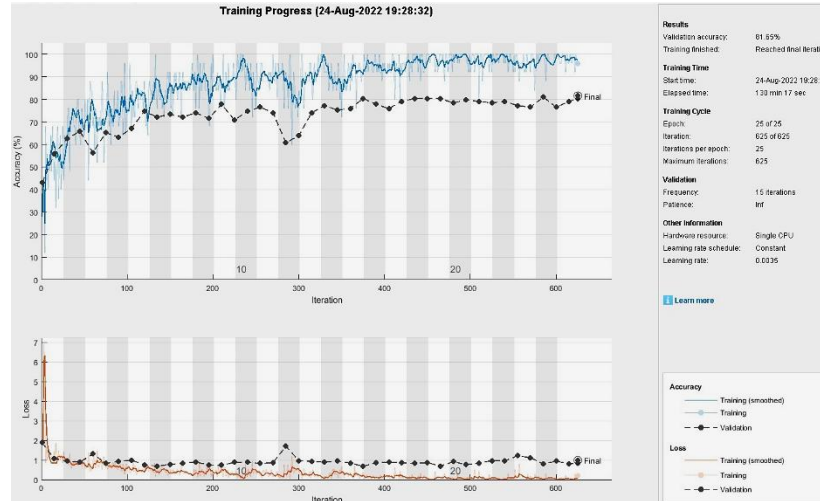
Figure 13: Training Graph of GoogleNet
