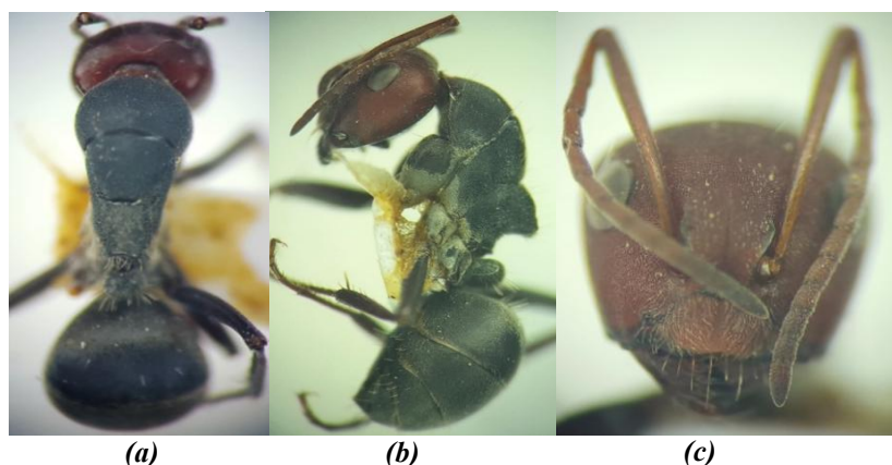
Figure 4: Camponotus sericeus . wide and compressed thorax, with scanting pubescence, meso-metanotal joint serrated (a), posteriorly excavated metanotum, pedicel with circular node, legs without prismatic tibia, abdomen wider and globe shaped (b), head broader and bulky, mandible with 5 teeth, clypeus tectiform with medially emarginated fore border(c).
