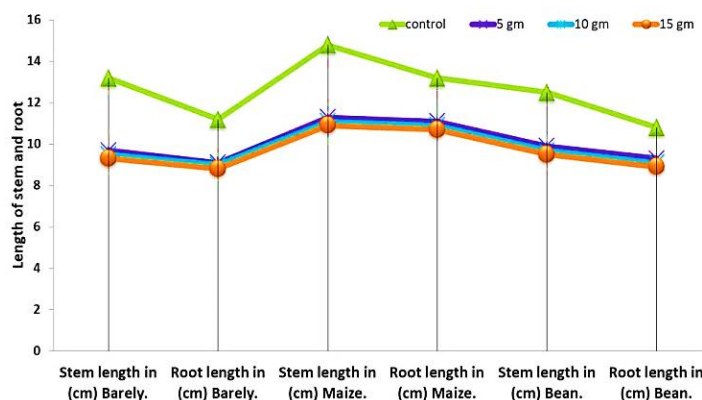
Figure 1: Effect of A. lebbbeck leaf powder on test crop stem and root length.
