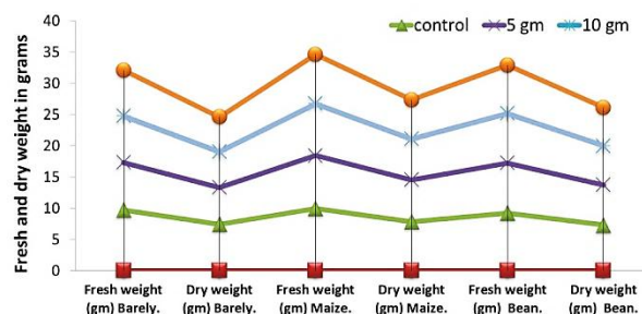
Figure 3: Impact of A. lebbbeck leaf powder on the dry and fresh biomass of test crops.
