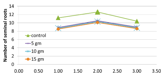
Figure 2: Impact of A. lebbbeck leaf powder on the root number of selected crops.
